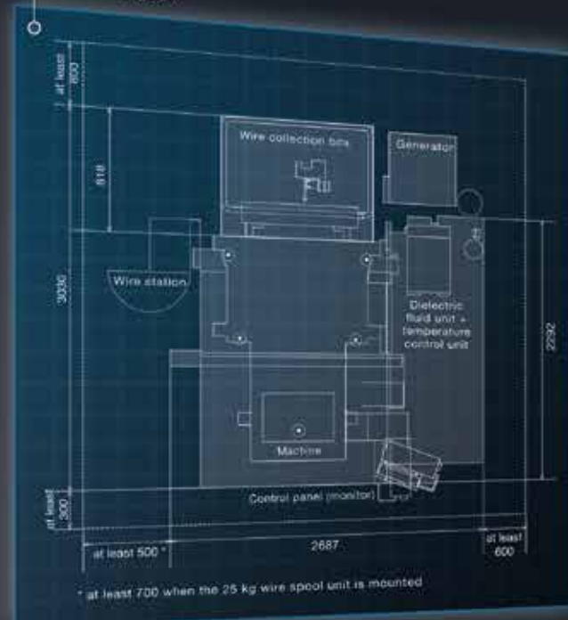
Machine plan
